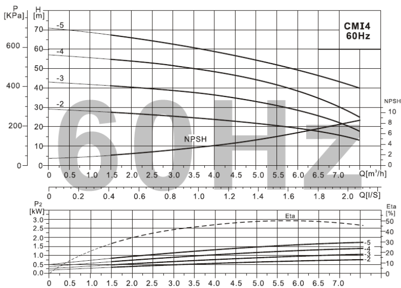
Curve Performance
