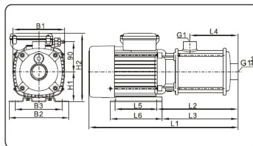
Installation Sketch
