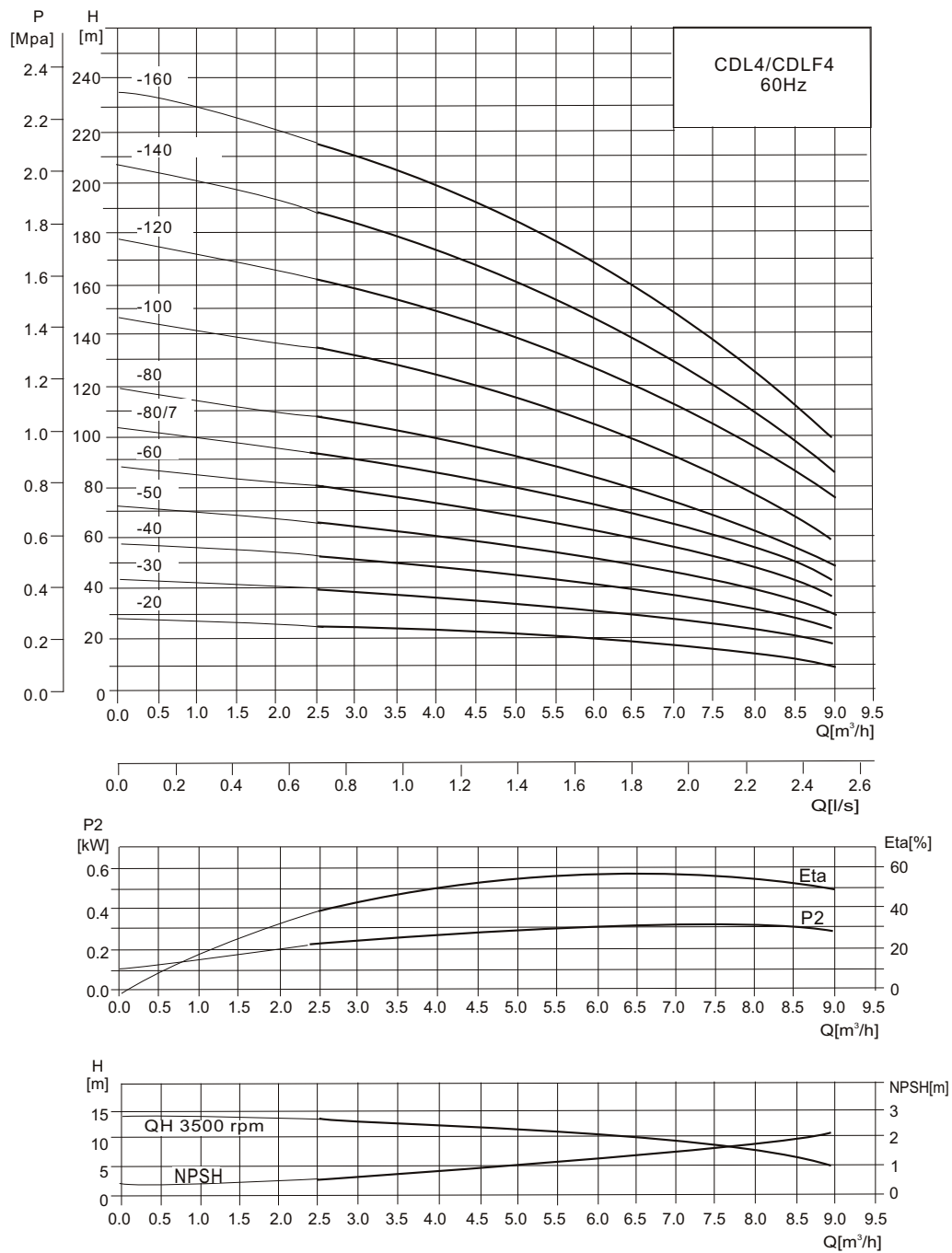
Performance curve
